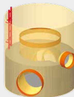
Stormwater overflow, spring pot
