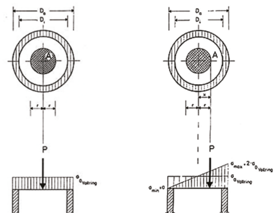
Centric loading
